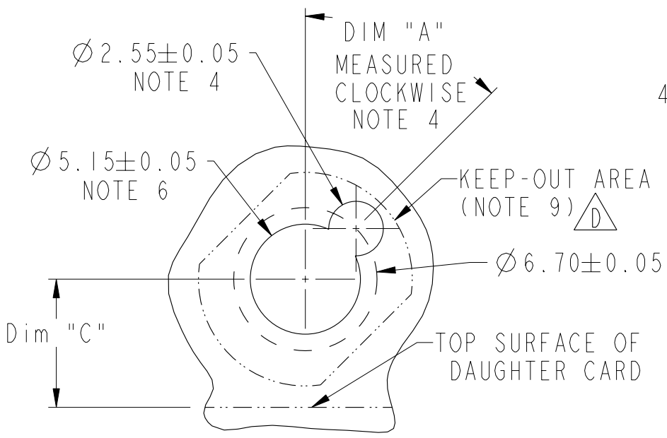
RECOMMENDED PCB LAYOUT (DRILLING) NOTES 4, 5 & 6 SCALE 4:1
